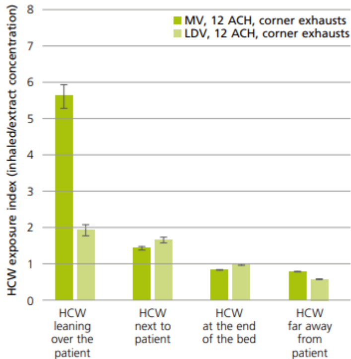
Figure 3 HCW exposure to patient's exhalation, by position and ventilation type. (Black whiskers represent standard error of the average exposure.)
