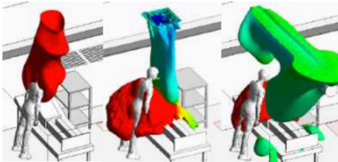
Figure 6 CFD simulation showing HCW exposure to patient's exhalation with mixing (left), local downward (centre) and zonal downward (right) ventilation. Exhaled air is shown as envelopes of constant concentration (red) and the flow of supply air as envelopes of constant velocity color-coded with concentration (blue and green represent low concentrations).
