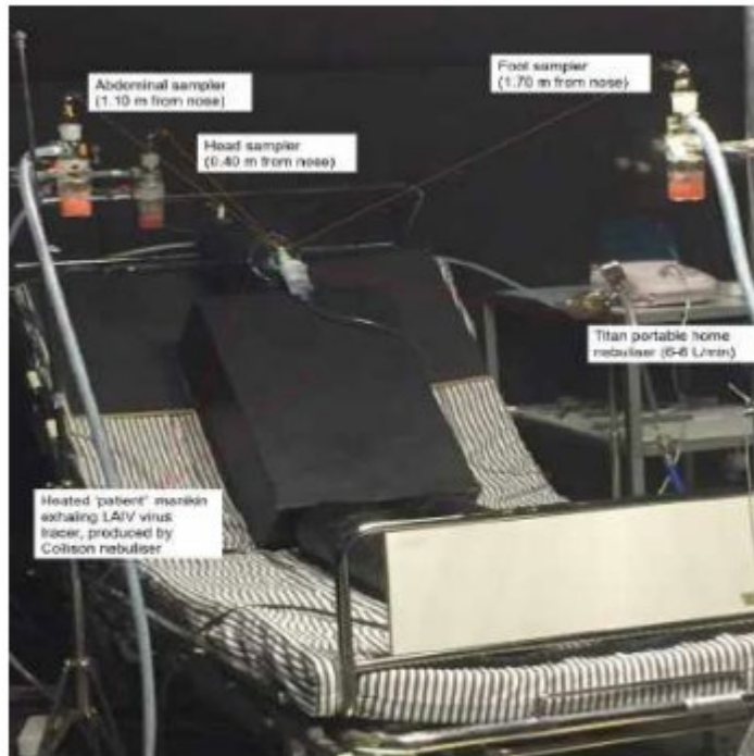
Figure 4 The experimental set-up to simulate HCW exposure to aerosol transmission when a patient is using a nebuliser mask.
