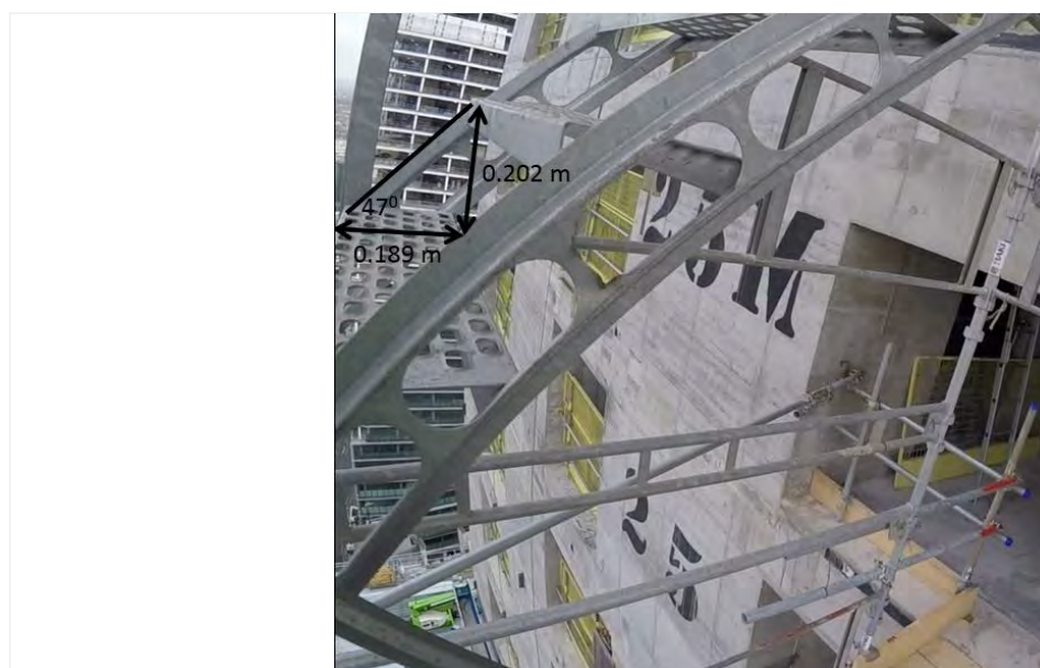
Figure 97. Tread and riser dimensions for the temporary scaffold dogleg stairs used in Trials 2 and 4.
