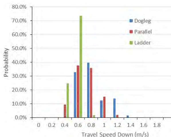
Figure 121. Comparison of descent travel speeds for the dogleg and parallel temporary scaffold stairs and ladders.
