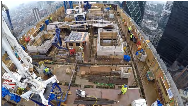
(a) View of top deck of slipform.
