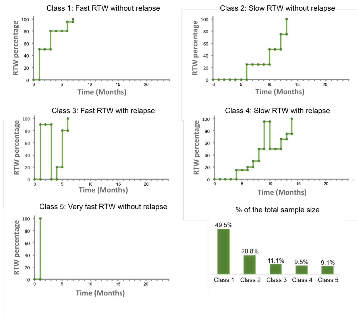
Figure 1. One example of a typical RTW trajectory per latent class of the five-class model (x-axis shows 24 months).
