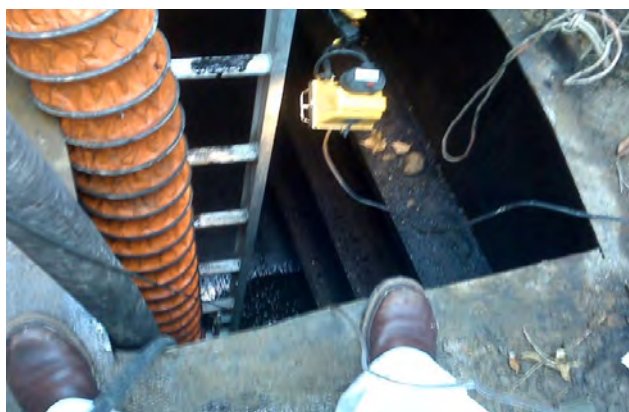
Figure 1. Ventilation hoses provide air and exhaust toxic vapors during confined space entry. The use of a guardrail would also be necessary to protect workers from potential falls.
