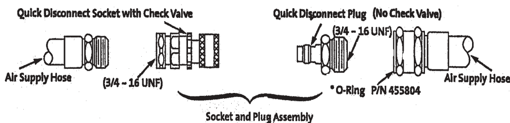
Figure 1. Quick Connector Diagram
