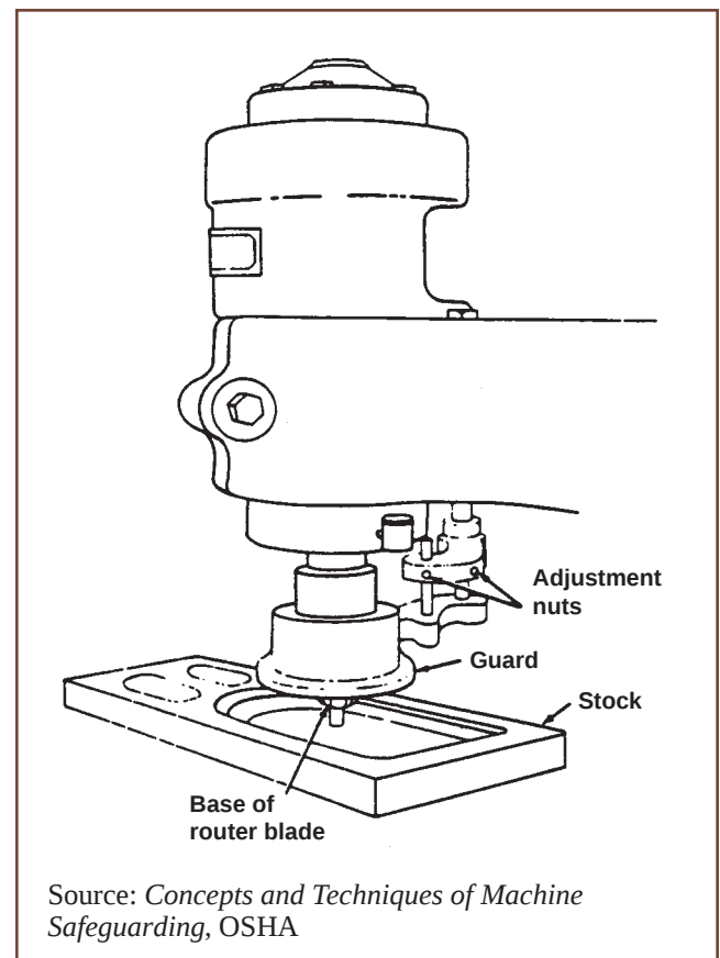
Figure 22. Router with Adjustable Tool Guard
