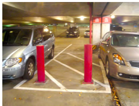
Figure 9.11. Floor striping indicates a FHC access path in a parking garage. Bollards provide vehicle impact protection. Bright signs at the top of the columns help firefighters locate the FHC.
