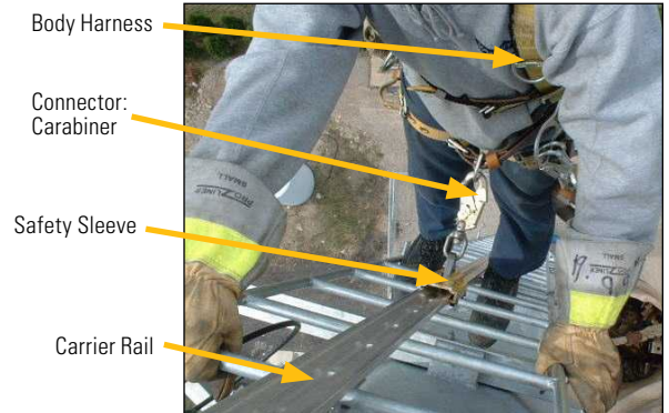
Figure 1: Components (parts) of a ladder safety device [fall protection equipment].
